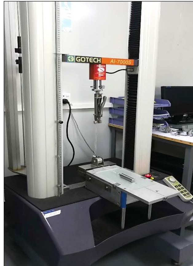
Tensile Strength Test for woven fabrics and leather
